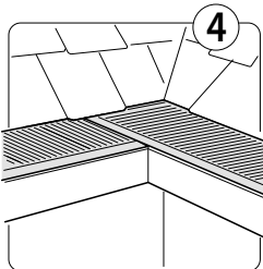
This is a completed inside corner. For heavy rain flow areas, you may need to add rain diverters.
