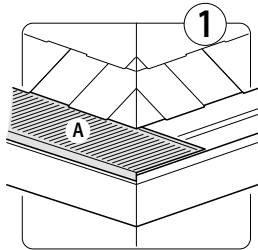
Place piece A along the outside corner.
