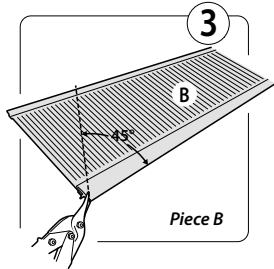
Cut piece B at a 45° angle.
